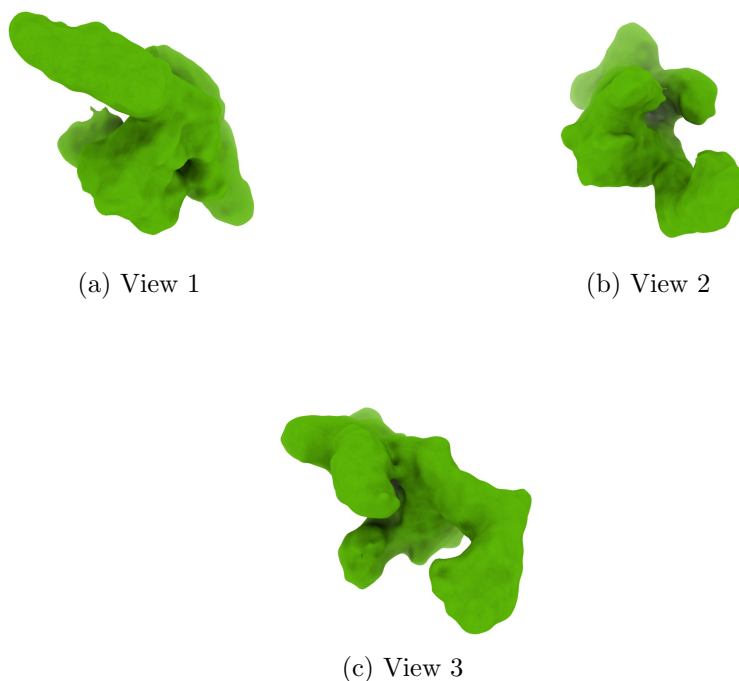
Figure 4: Isosurface at threshold=0.012400. Views generated by ChimeraX at a the following X, Y, Z angles: View 1 (0, -90, -90), View 2 (-90, 0, -90), View 3 (0, 0, 0).
