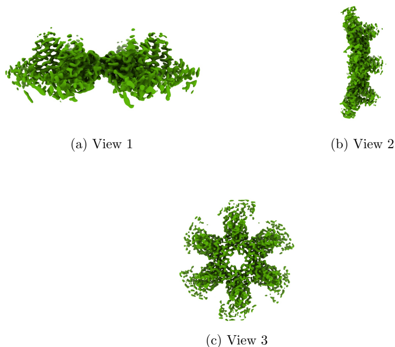
Figure 4: Isosurface at threshold=0.010200. Views generated by ChimeraX at a the following X, Y, Z angles: View 1 (0, -90, -90), View 2 (-90, 0, -90), View 3 (0, 0, 0).
