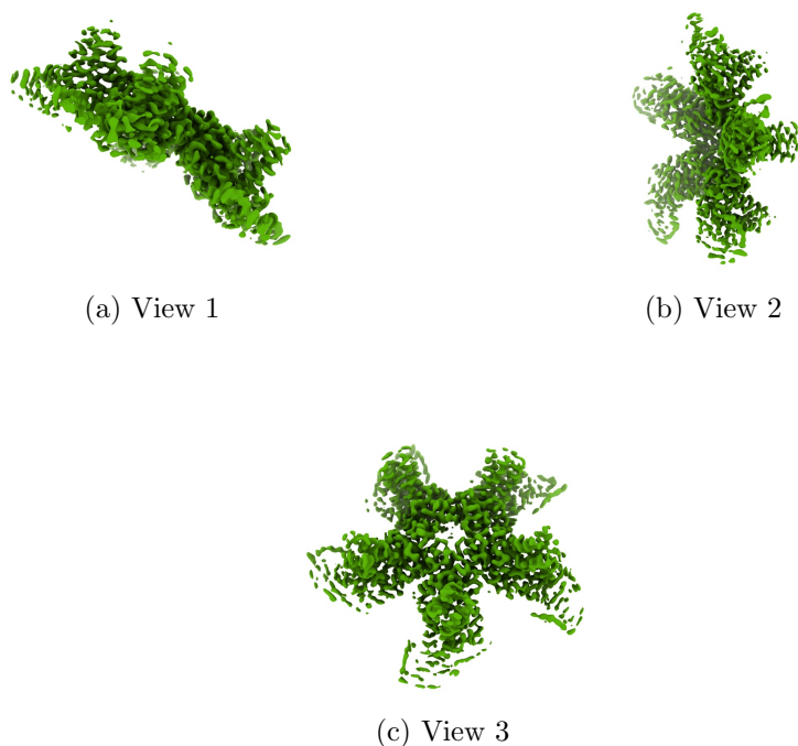
Figure 4: Isosurface at threshold=0.018400. Views generated by ChimeraX at a the following X, Y, Z angles: View 1 (0, -90, -90), View 2 (-90, 0, -90), View 3 (0, 0, 0).
