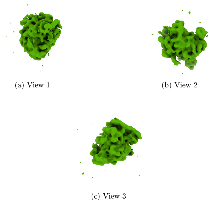
Figure 4: Isosurface at threshold=24.600000. Views generated by ChimeraX at a the following X, Y, Z angles: View 1 (0, -90, -90), View 2 (-90, 0, -90), View 3 (0, 0, 0).
