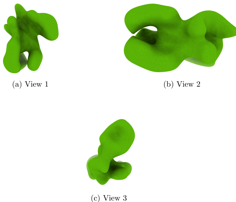
Figure 4: Isosurface at threshold=0.028800. Views generated by ChimeraX at a the following X, Y, Z angles: View 1 (0, -90, -90), View 2 (-90, 0, -90), View 3 (0, 0, 0).
