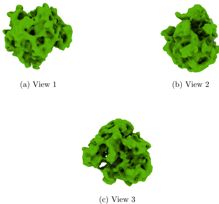
Figure 4: Isosurface at threshold=2.170000. Views generated by ChimeraX at a the following X, Y, Z angles: View 1 (0, -90, -90), View 2 (-90, 0, -90), View 3 (0, 0, 0).
