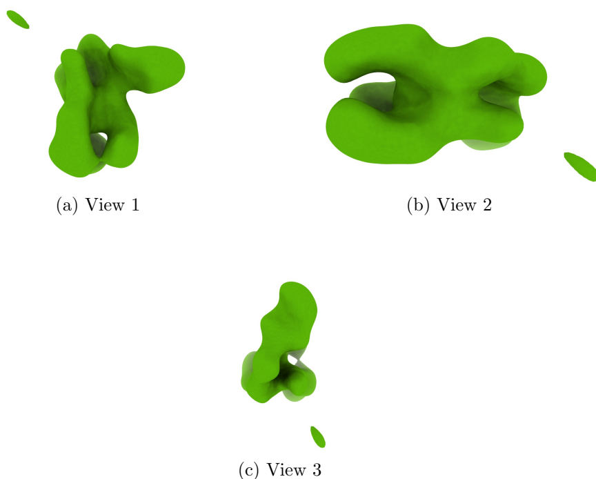
Figure 4: Isosurface at threshold=0.024900. Views generated by ChimeraX at the following X, Y, Z angles: View 1 (0, -90, -90), View 2 (-90, 0, -90), View 3 (0, 0, 0).
