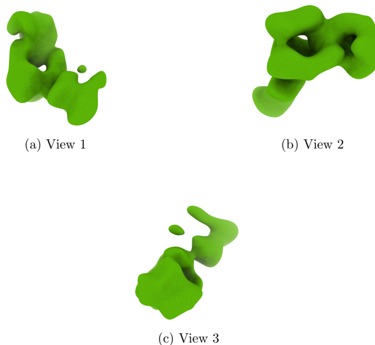
Figure 4: Isosurface at threshold=0.021300. Views generated by ChimeraX at a the following X, Y, Z angles: View 1 (0, -90, -90), View 2 (-90, 0, -90), View 3 (0, 0, 0).
