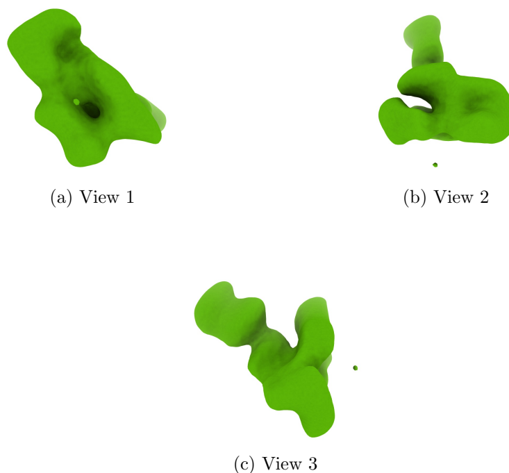
Figure 4: Isosurface at threshold=0.018600. Views generated by ChimeraX at a the following X, Y, Z angles: View 1 (0, -90, -90), View 2 (-90, 0, -90), View 3 (0, 0, 0).
