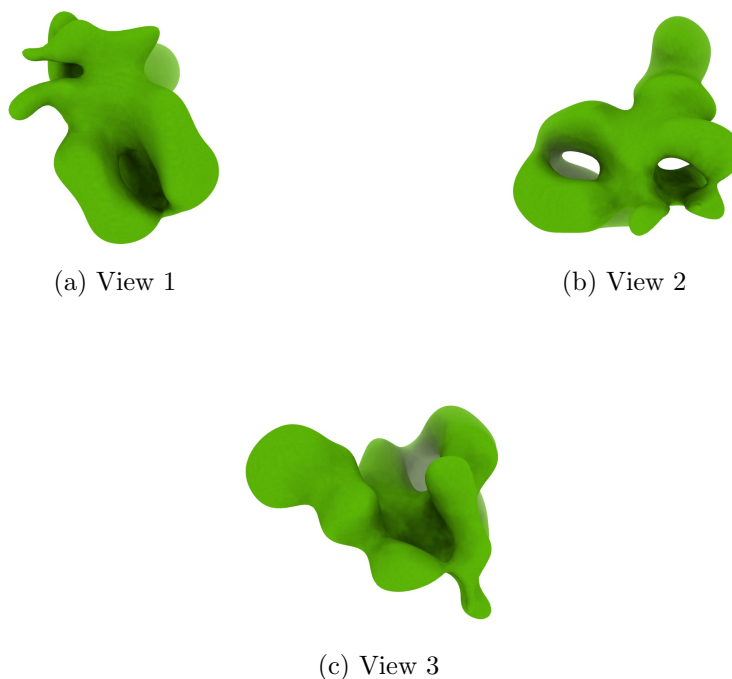
Figure 4: Isosurface at threshold=0.027600. Views generated by ChimeraX at a the following X, Y, Z angles: View 1 (0, -90, -90), View 2 (-90, 0, -90), View 3 (0, 0, 0).
