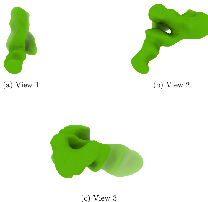
Figure 4: Isosurface at threshold=0.018200. Views generated by ChimeraX at a the following X, Y, Z angles: View 1 (0, -90, -90), View 2 (-90, 0, -90), View 3 (0, 0, 0).
