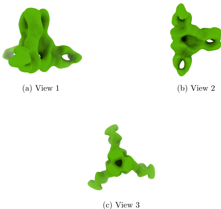
Figure 4: Isosurface at threshold=0.011100. Views generated by ChimeraX at a the following X, Y, Z angles: View 1 (0, -90, -90), View 2 (-90, 0, -90), View 3 (0, 0, 0).
