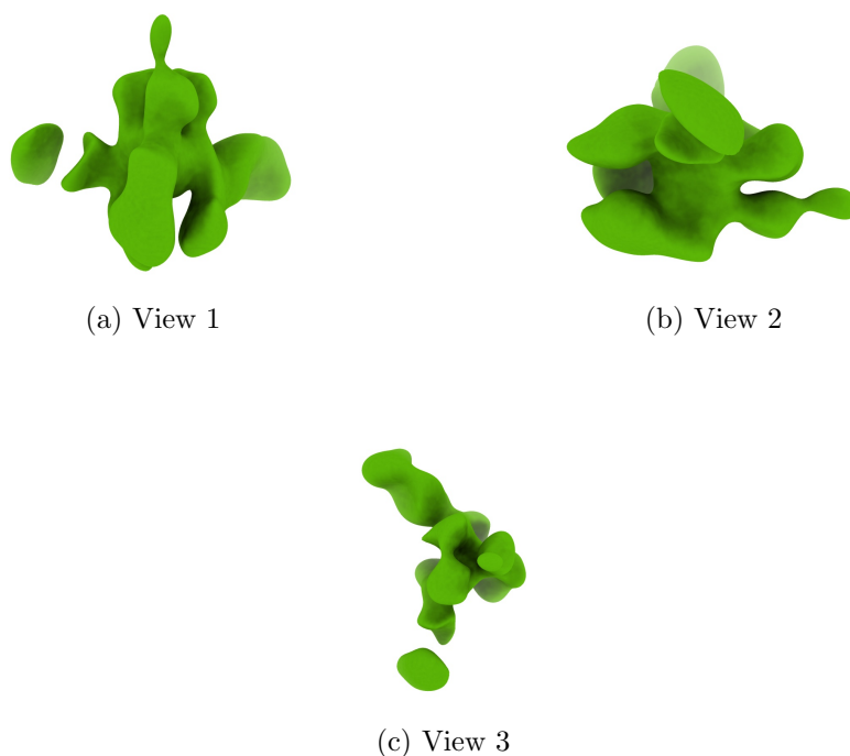
Figure 4: Isosurface at threshold=0.015500. Views generated by ChimeraX at a the following X, Y, Z angles: View 1 (0, -90, -90), View 2 (-90, 0, -90), View 3 (0, 0, 0).
