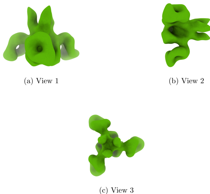
Figure 4: Isosurface at threshold=0.012200. Views generated by ChimeraX at a the following X, Y, Z angles: View 1 (0, -90, -90), View 2 (-90, 0, -90), View 3 (0, 0, 0).
