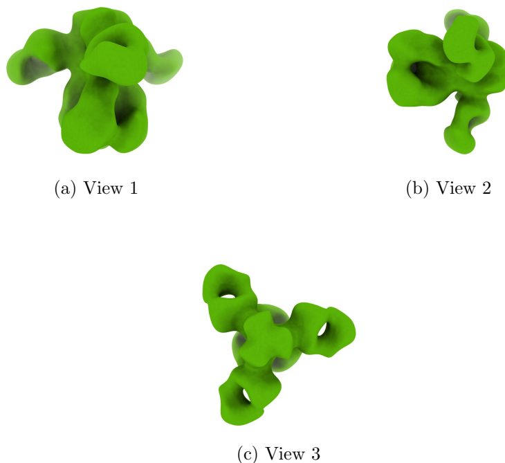
Figure 4: Isosurface at threshold=0.010300. Views generated by ChimeraX at a the following X, Y, Z angles: View 1 (0, -90, -90), View 2 (-90, 0, -90), View 3 (0, 0, 0).
