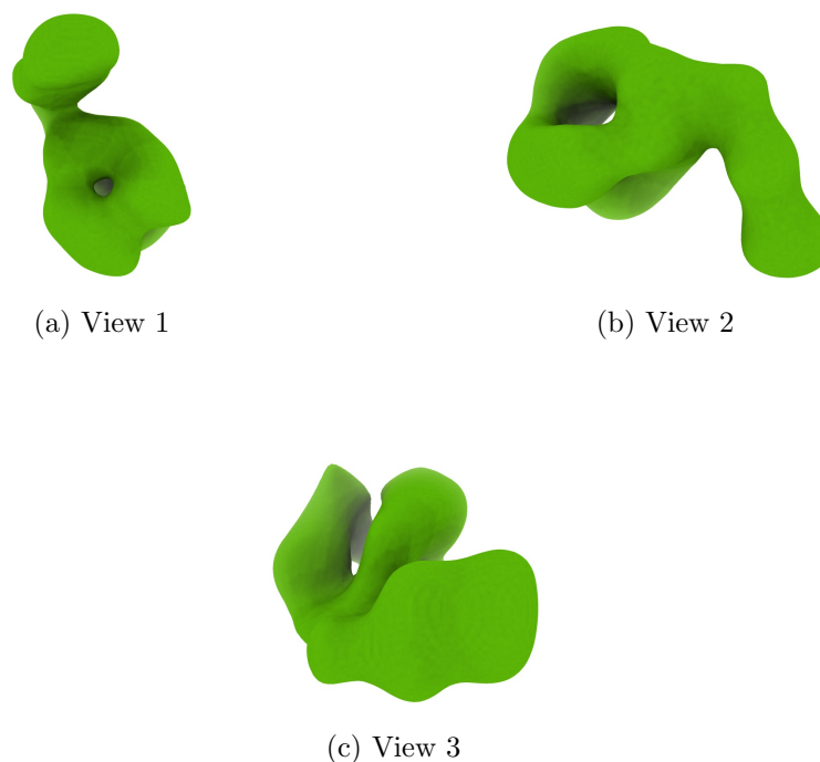
Figure 4: Isosurface at threshold=0.027800. Views generated by ChimeraX at a the following X, Y, Z angles: View 1 (0, -90, -90), View 2 (-90, 0, -90), View 3 (0, 0, 0).
