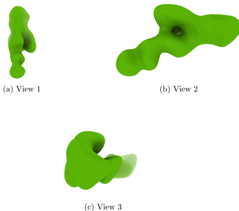
Figure 4: Isosurface at threshold=0.031800. Views generated by ChimeraX at the following X, Y, Z angles: View 1 (0, -90, -90), View 2 (-90, 0, -90), View 3 (0, 0, 0).
