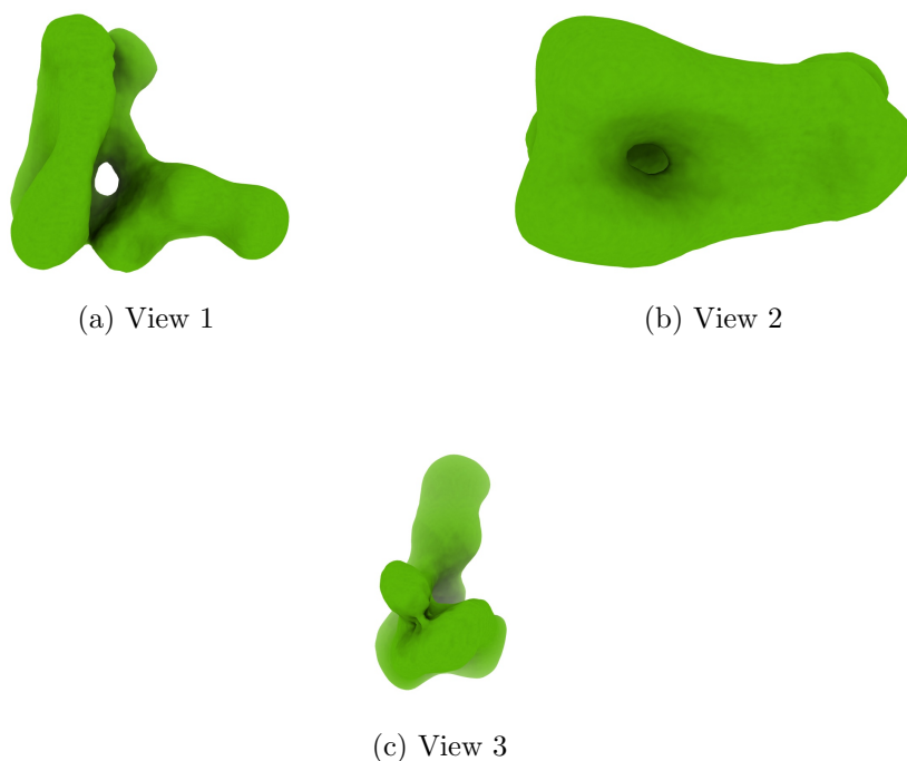
Figure 4: Isosurface at threshold=0.029700. Views generated by ChimeraX at a the following X, Y, Z angles: View 1 (0, -90, -90), View 2 (-90, 0, -90), View 3 (0, 0, 0).
