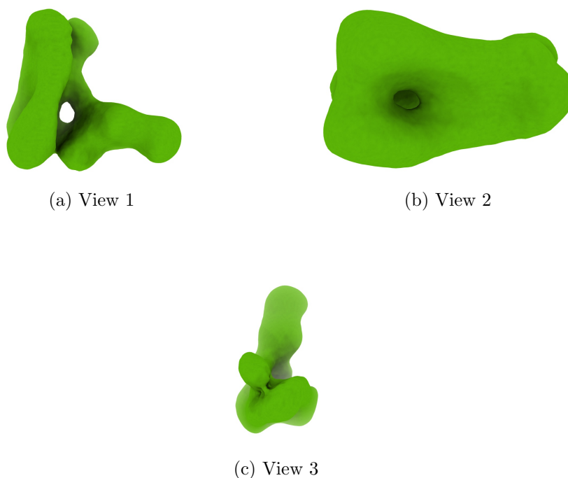
Figure 4: Isosurface at threshold=0.029700. Views generated by ChimeraX at a the following X, Y, Z angles: View 1 (0, -90, -90), View 2 (-90, 0, -90), View 3 (0, 0, 0).
