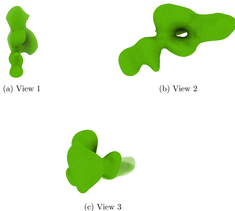
Figure 4: Isosurface at threshold=0.029300. Views generated by ChimeraX at a the following X, Y, Z angles: View 1 (0, -90, -90), View 2 (-90, 0, -90), View 3 (0, 0, 0).
