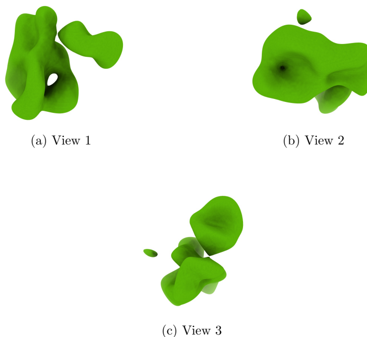
Figure 4: Isosurface at threshold=0.026300. Views generated by ChimeraX at a the following X, Y, Z angles: View 1 (0, -90, -90), View 2 (-90, 0, -90), View 3 (0, 0, 0).
