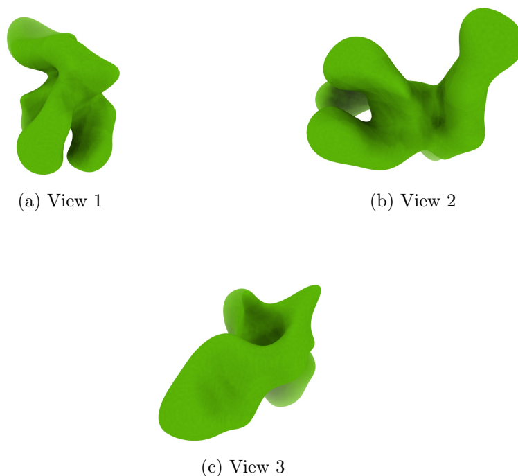
Figure 4: Isosurface at threshold=0.025900. Views generated by ChimeraX at a the following X, Y, Z angles: View 1 (0, -90, -90), View 2 (-90, 0, -90), View 3 (0, 0, 0).
