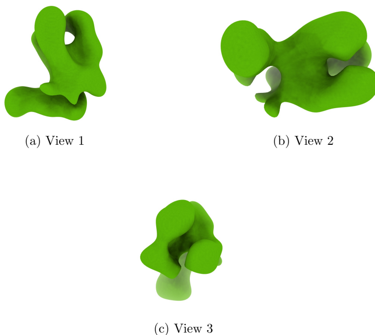
Figure 4: Isosurface at threshold=0.032200. Views generated by ChimeraX at a the following X, Y, Z angles: View 1 (0, -90, -90), View 2 (-90, 0, -90), View 3 (0, 0, 0).
