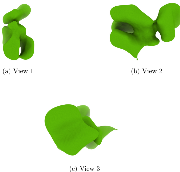
Figure 4: Isosurface at threshold=0.026900. Views generated by ChimeraX at a the following X, Y, Z angles: View 1 (0, -90, -90), View 2 (-90, 0, -90), View 3 (0, 0, 0).
