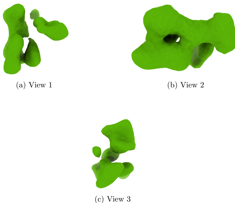
Figure 4: Isosurface at threshold=0.026600. Views generated by ChimeraX at a the following X, Y, Z angles: View 1 (0, -90, -90), View 2 (-90, 0, -90), View 3 (0, 0, 0).
