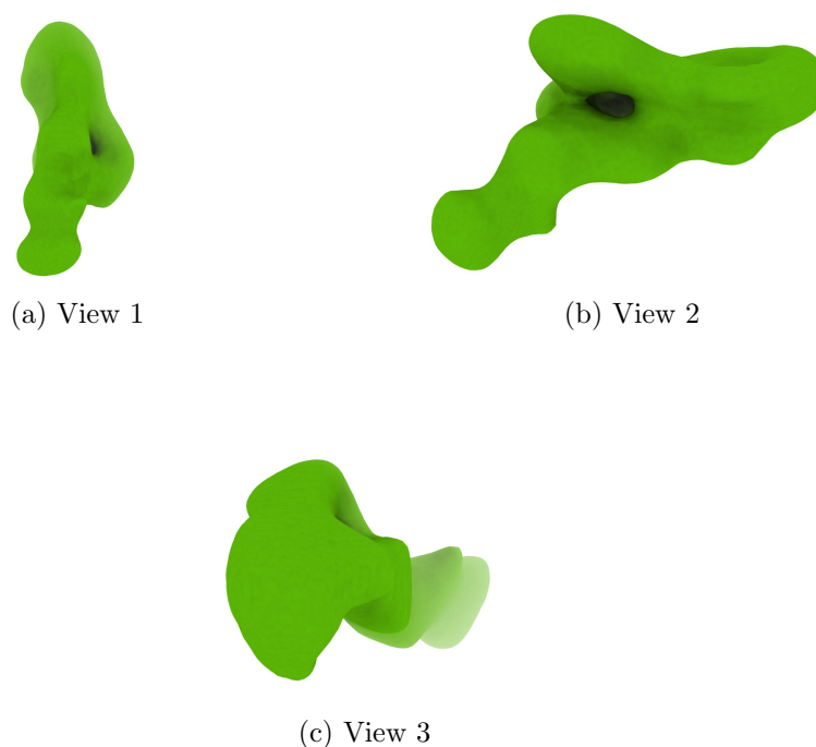
Figure 4: Isosurface at threshold=0.026900. Views generated by ChimeraX at a the following X, Y, Z angles: View 1 (0, -90, -90), View 2 (-90, 0, -90), View 3 (0, 0, 0).
