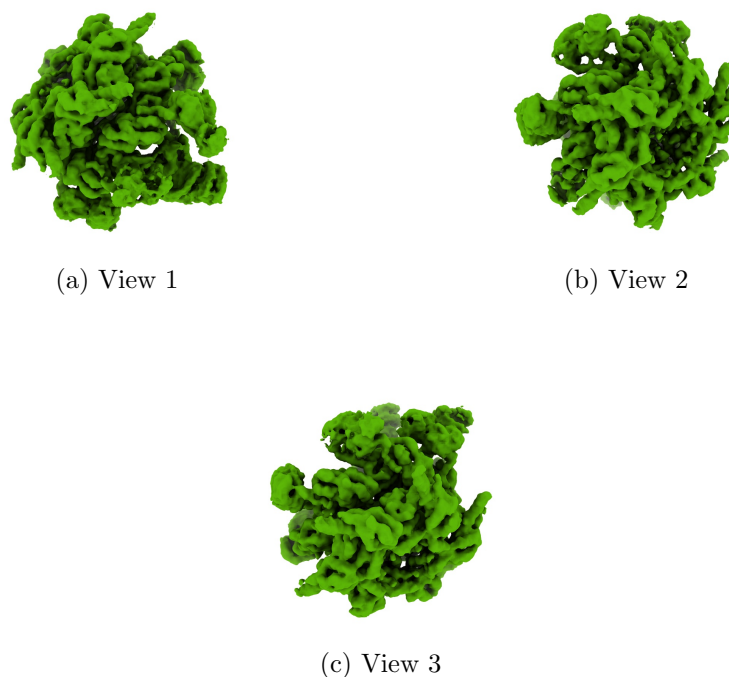
Figure 4: Isosurface at threshold=0.014900. Views generated by ChimeraX at a the following X, Y, Z angles: View 1 (0, -90, -90), View 2 (-90, 0, -90), View 3 (0, 0, 0).
