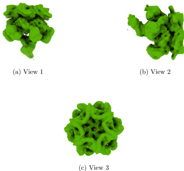
Figure 4: Isosurface at threshold=0.008200. Views generated by ChimeraX at a the following X, Y, Z angles: View 1 (0, -90, -90), View 2 (-90, 0, -90), View 3 (0, 0, 0).
