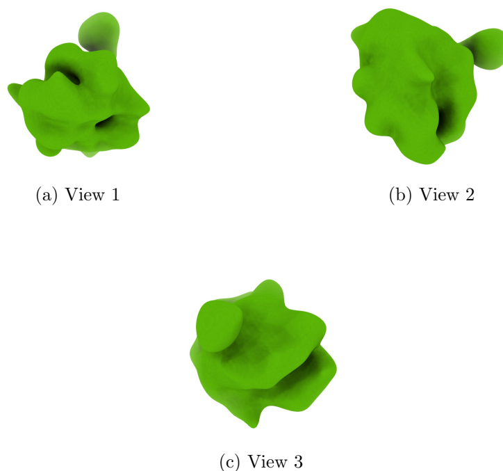
Figure 4: Isosurface at threshold=0.066400. Views generated by ChimeraX at a the following X, Y, Z angles: View 1 (0, -90, -90), View 2 (-90, 0, -90), View 3 (0, 0, 0).
