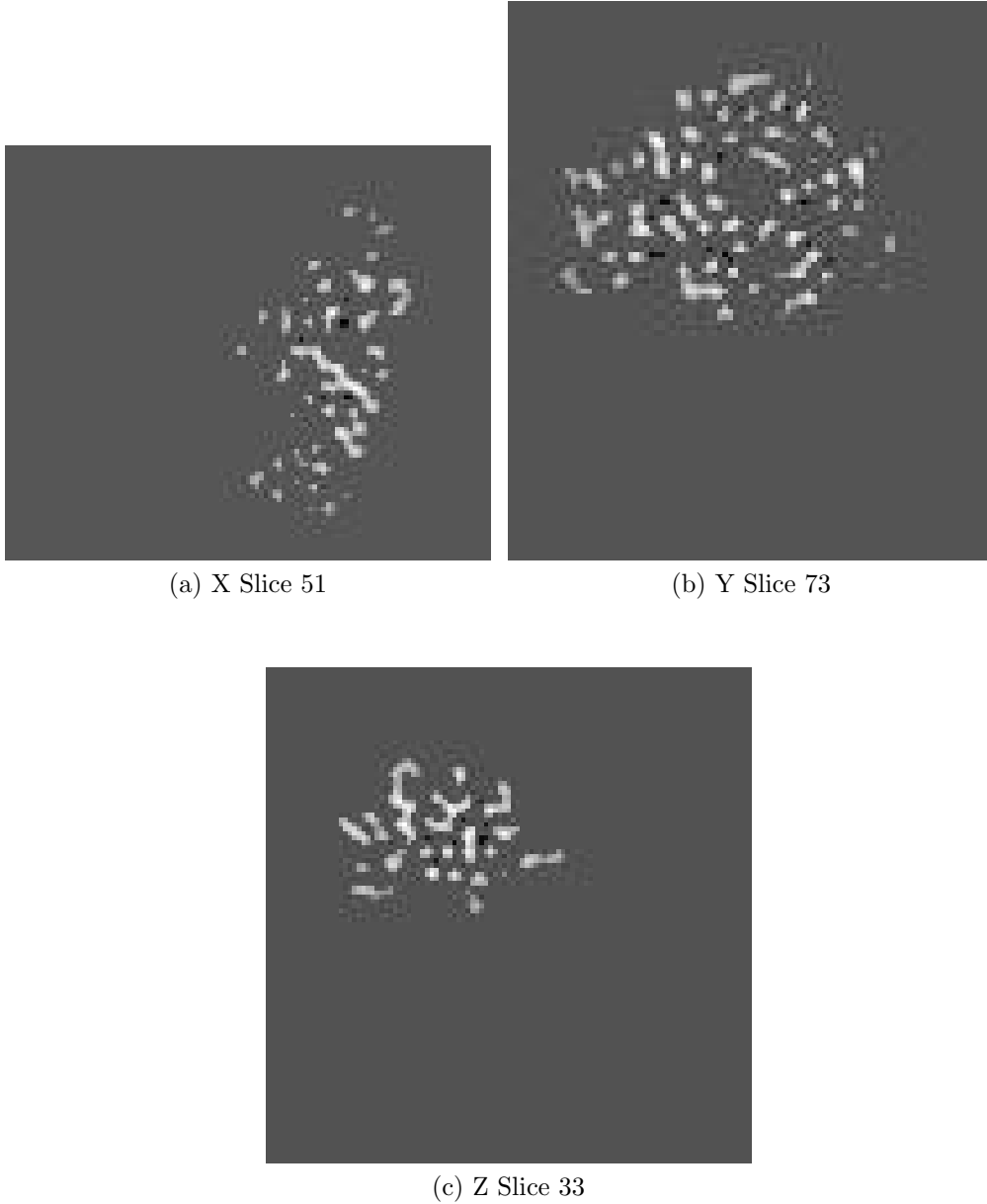
Figure 9: Maximum variance slices in the three dimensions of the parts of the background beyond 5\sigma
