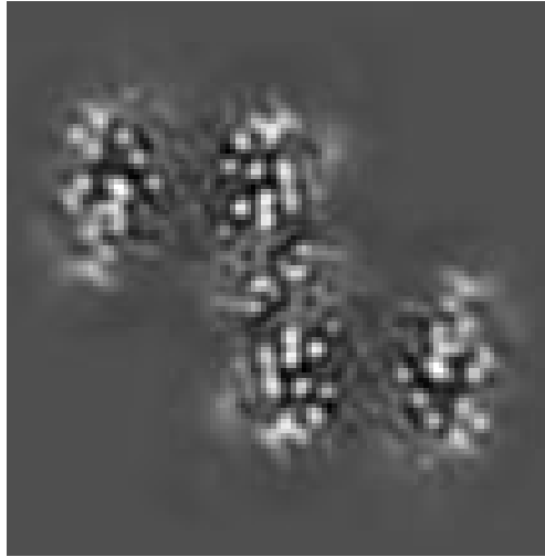
(c) Z Slice 46
