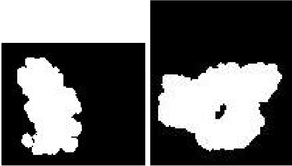
(a) X Slice 58
