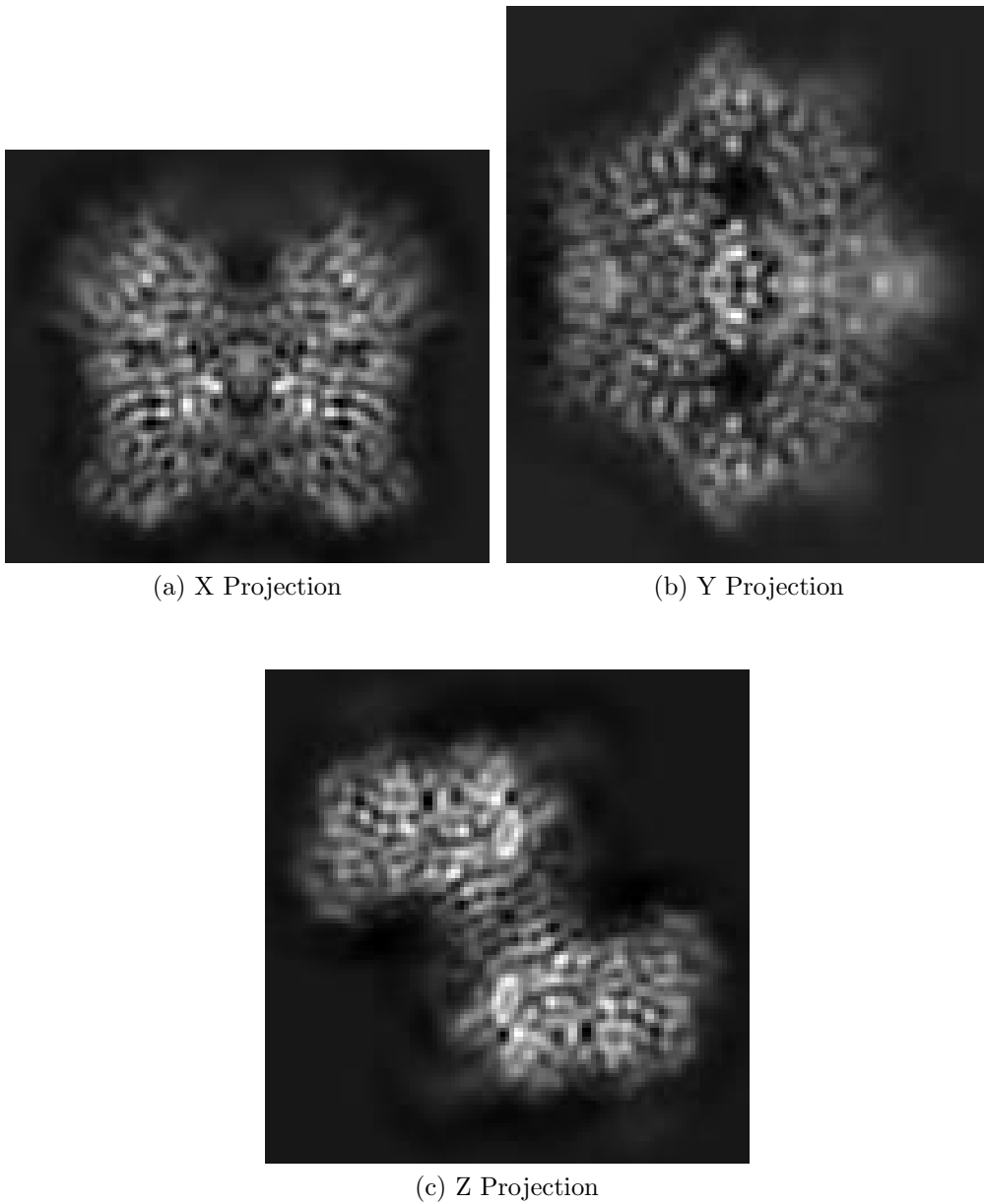
Figure 3: Projections in the three dimensions
