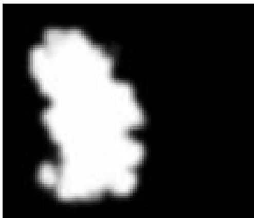
(a) X Slice 58
