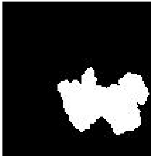
(c) Z Slice 40
