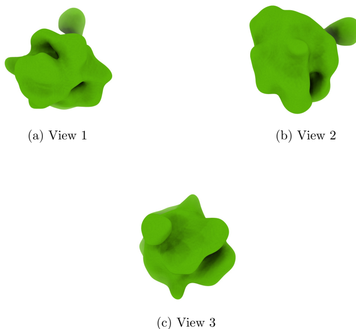
Figure 4: Isosurface at threshold=0.066600. Views generated by ChimeraX at a the following X, Y, Z angles: View 1 (0, -90, -90), View 2 (-90, 0, -90), View 3 (0, 0, 0).
