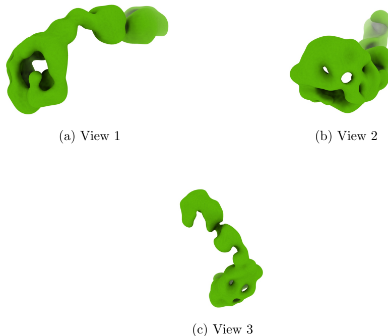
Figure 4: Isosurface at threshold=0.048100. Views generated by ChimeraX at a the following X, Y, Z angles: View 1 (0, -90, -90), View 2 (-90, 0, -90), View 3 (0, 0, 0).
