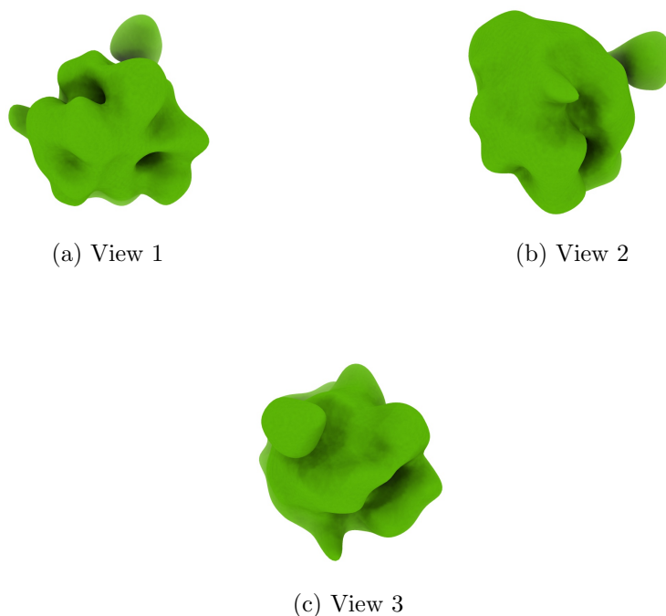
Figure 4: Isosurface at threshold=0.072300. Views generated by ChimeraX at a the following X, Y, Z angles: View 1 (0, -90, -90), View 2 (-90, 0, -90), View 3 (0, 0, 0).
