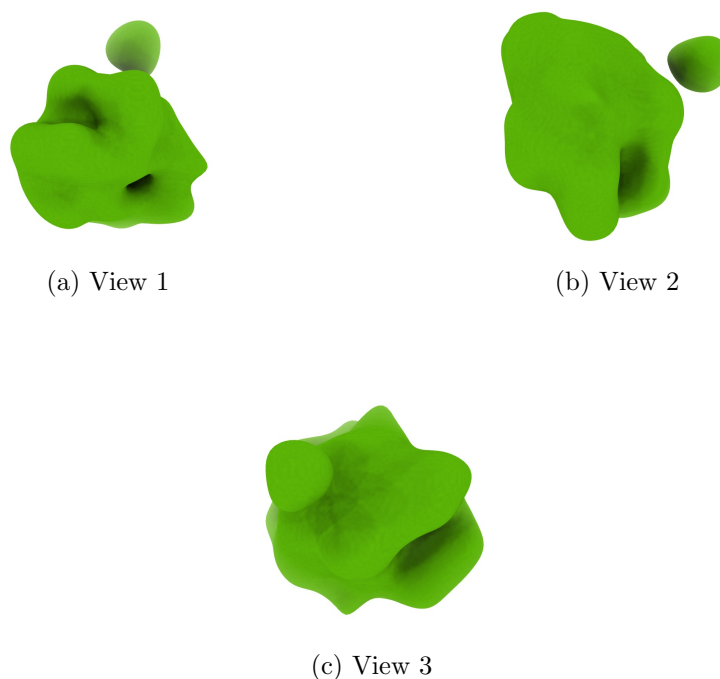
Figure 4: Isosurface at threshold=0.085000. Views generated by ChimeraX at a the following X, Y, Z angles: View 1 (0, -90, -90), View 2 (-90, 0, -90), View 3 (0, 0, 0).
