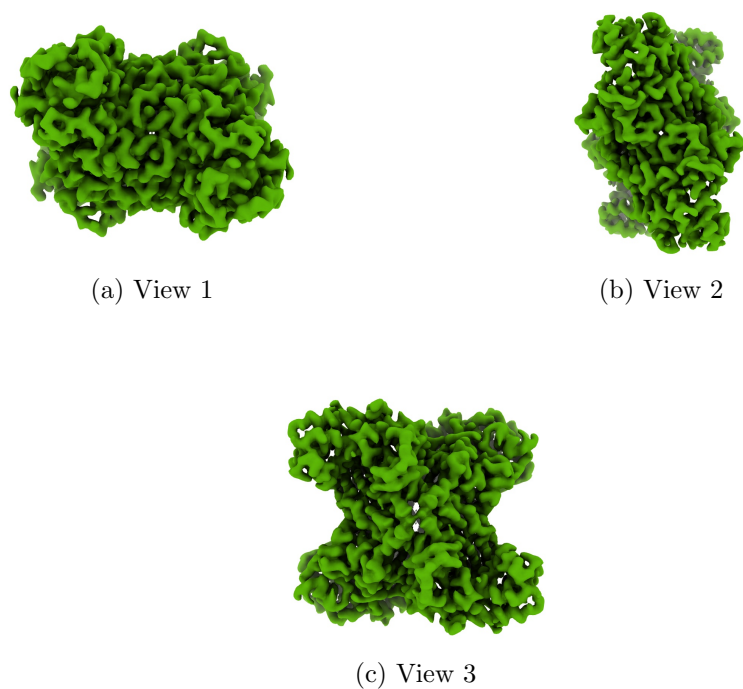
Figure 4: Isosurface at threshold=0.212000. Views generated by ChimeraX at a the following X, Y, Z angles: View 1 (0, -90, -90), View 2 (-90, 0, -90), View 3 (0, 0, 0).
