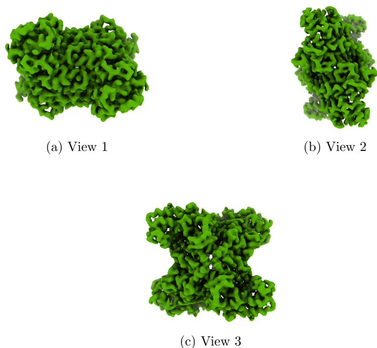
Figure 4: Isosurface at threshold=0.212000. Views generated by ChimeraX at the following X, Y, Z angles: View 1 (0, -90, -90), View 2 (-90, 0, -90), View 3 (0, 0, 0).
