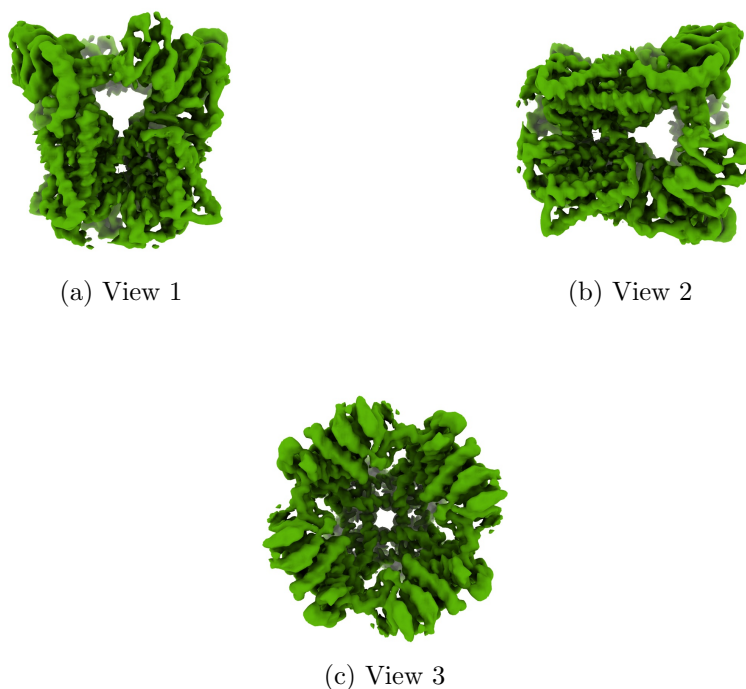
Figure 4: Isosurface at threshold=0.307000. Views generated by ChimeraX at a the following X, Y, Z angles: View 1 (0, -90, -90), View 2 (-90, 0, -90), View 3 (0, 0, 0).
