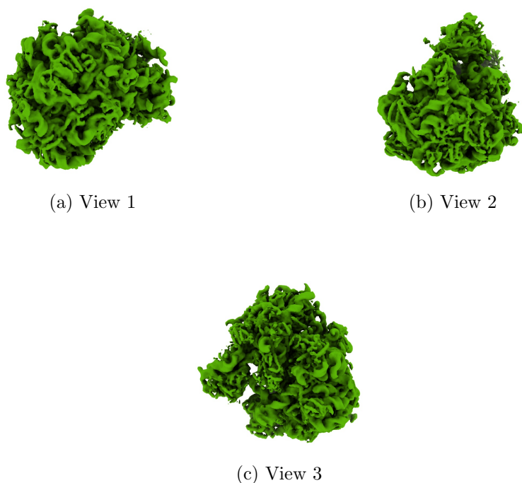
Figure 4: Isosurface at threshold=1.580000. Views generated by ChimeraX at a the following X, Y, Z angles: View 1 (0, -90, -90), View 2 (-90, 0, -90), View 3 (0, 0, 0).
