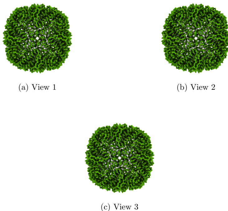
Figure 4: Isosurface at threshold=0.600000. Views generated by ChimeraX at the following X, Y, Z angles: View 1 (0, -90, -90), View 2 (-90, 0, -90), View 3 (0, 0, 0).
