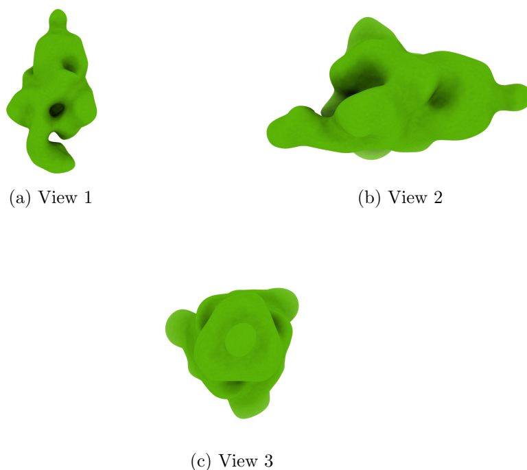
Figure 4: Isosurface at threshold=1.150000. Views generated by ChimeraX at a the following X, Y, Z angles: View 1 (0, -90, -90), View 2 (-90, 0, -90), View 3 (0, 0, 0).
