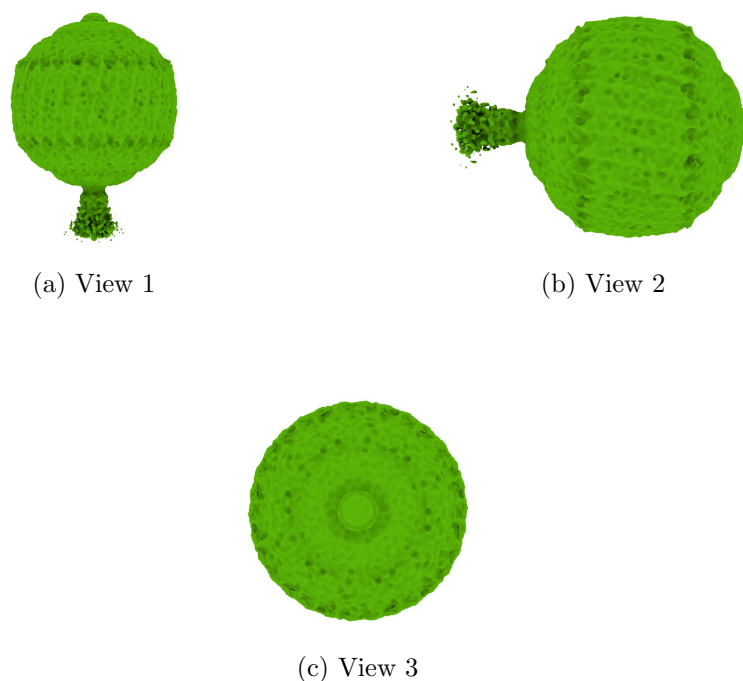
Figure 4: Isosurface at threshold=6000.000000. Views generated by ChimeraX at the following X, Y, Z angles: View 1 (0, -90, -90), View 2 (-90, 0, -90), View 3 (0, 0, 0).
