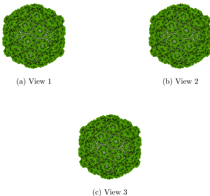
Figure 4: Isosurface at threshold=10000.000000. Views generated by ChimeraX at the following X, Y, Z angles: View 1 (0, -90, -90), View 2 (-90, 0, -90), View 3 (0, 0, 0).
