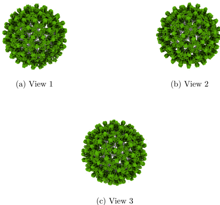
Figure 4: Isosurface at threshold=0.008070. Views generated by ChimeraX at a the following X, Y, Z angles: View 1 (0, -90, -90), View 2 (-90, 0, -90), View 3 (0, 0, 0).
