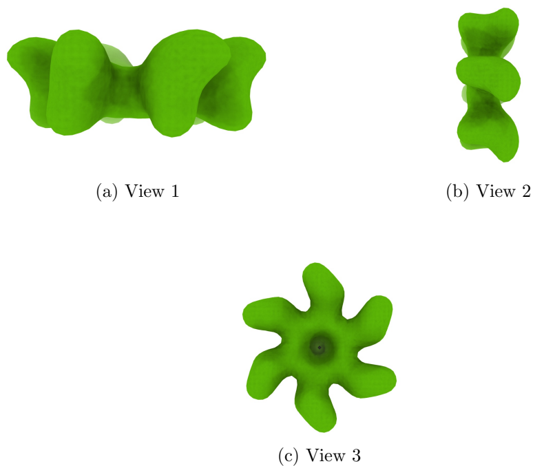
Figure 4: Isosurface at threshold=0.038400. Views generated by ChimeraX at a the following X, Y, Z angles: View 1 (0, -90, -90), View 2 (-90, 0, -90), View 3 (0, 0, 0).
