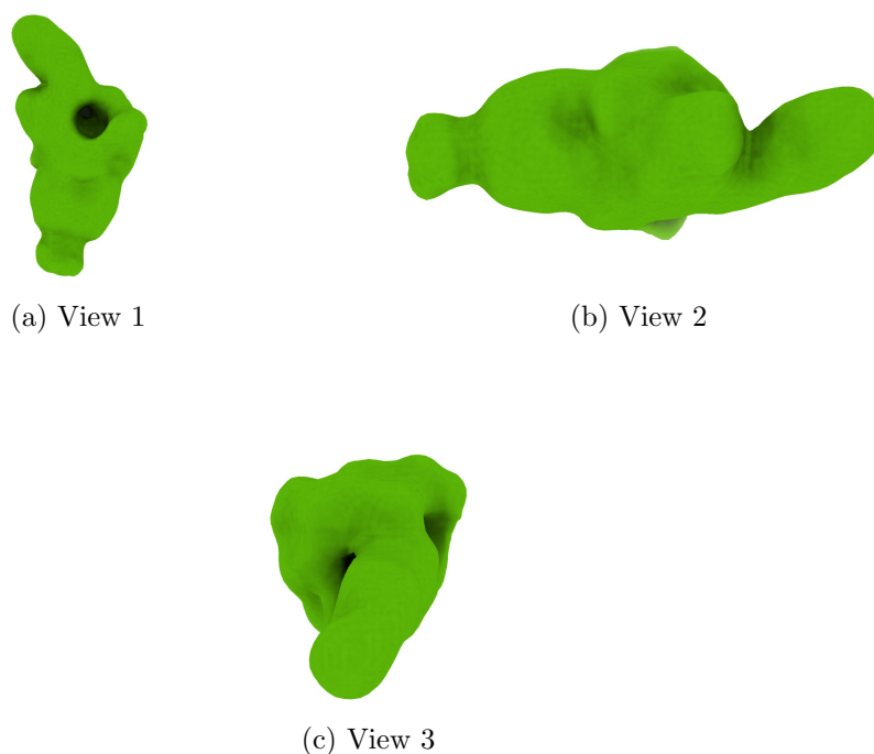
Figure 4: Isosurface at threshold=4.800000. Views generated by ChimeraX at a the following X, Y, Z angles: View 1 (0, -90, -90), View 2 (-90, 0, -90), View 3 (0, 0, 0).
