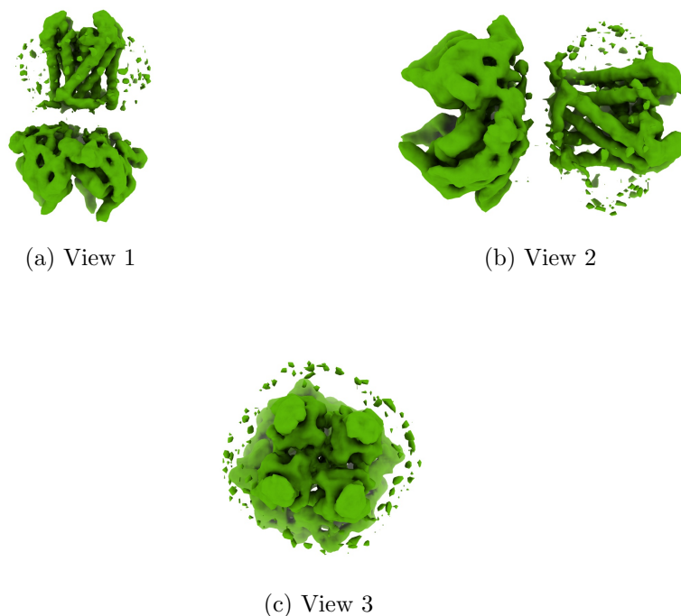
Figure 4: Isosurface at threshold=0.009400. Views generated by ChimeraX at a the following X, Y, Z angles: View 1 (0, -90, -90), View 2 (-90, 0, -90), View 3 (0, 0, 0).
