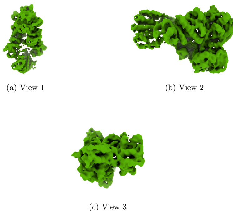
Figure 4: Isosurface at threshold=0.019000. Views generated by ChimeraX at a the following X, Y, Z angles: View 1 (0, -90, -90), View 2 (-90, 0, -90), View 3 (0, 0, 0).
