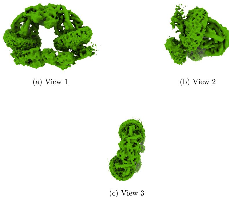
Figure 4: Isosurface at threshold=0.005500. Views generated by ChimeraX at a the following X, Y, Z angles: View 1 (0, -90, -90), View 2 (-90, 0, -90), View 3 (0, 0, 0).
