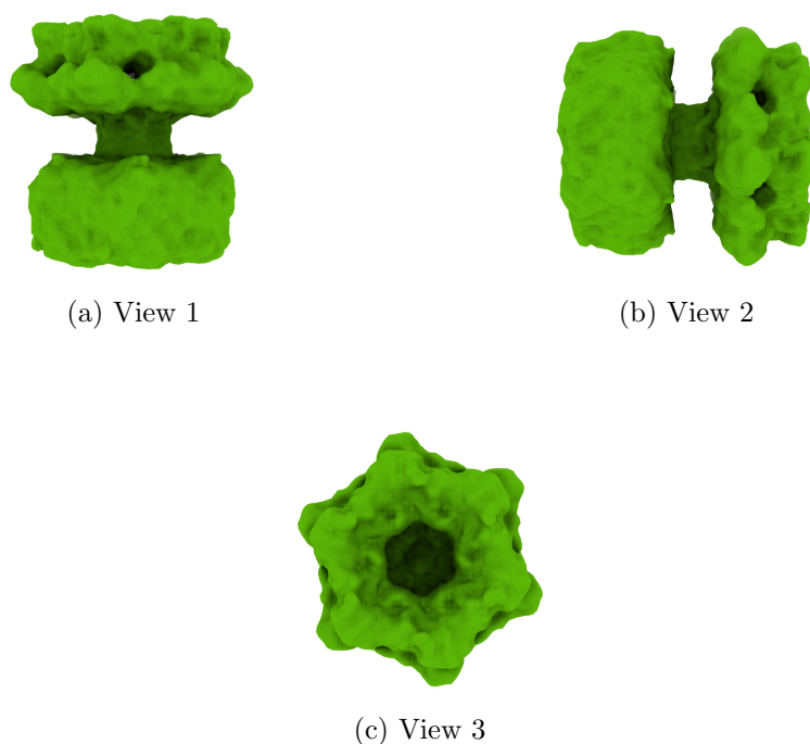
Figure 4: Isosurface at threshold=0.830000. Views generated by ChimeraX at a the following X, Y, Z angles: View 1 (0, -90, -90), View 2 (-90, 0, -90), View 3 (0, 0, 0).
