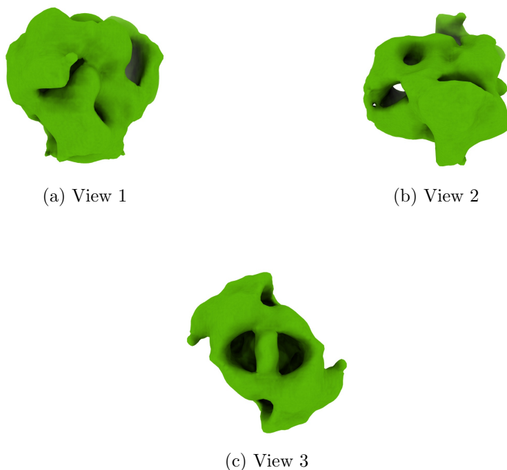
Figure 4: Isosurface at threshold=0.000500. Views generated by ChimeraX at a the following X, Y, Z angles: View 1 (0, -90, -90), View 2 (-90, 0, -90), View 3 (0, 0, 0).
